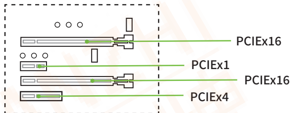
2-4 PCI Expansion Slot
